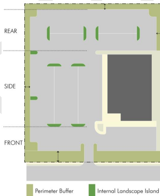
Figure 7-1 Parking Design
